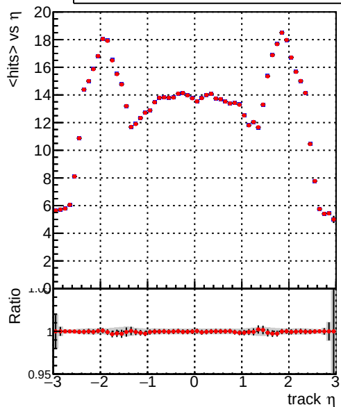
mean hits vs \eta Legend: DQM_TT_mkFit-DQM_old132 (blue line), DQM_TT_mkFit-DQM_new132 (red line)
