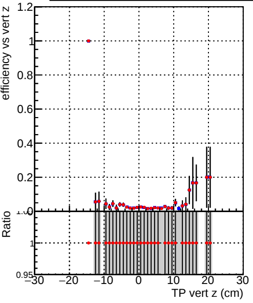
Efficiency vs TP vert z (cm) Legend: DQM_TT_mkFit-DQM_old132 (blue squares) DQM_TT_mkFit-DQM_new132 (red diamonds)
