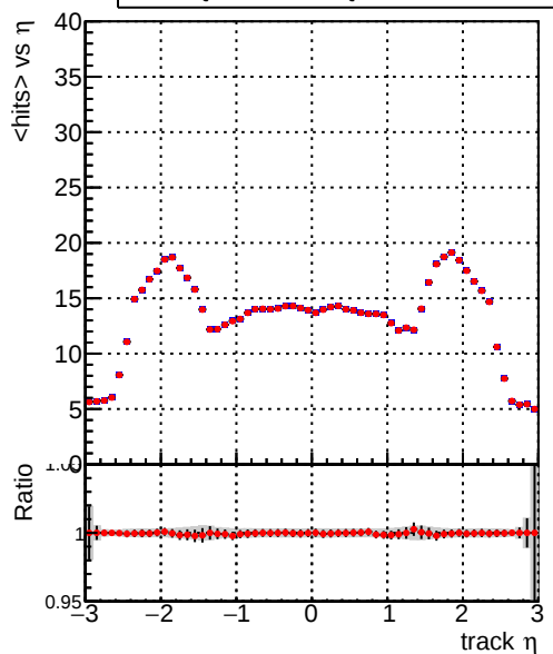
mean hit — DQM_TT_mkFit-DQM_old132 — DQM_TT_mkFit-DQM_new132
