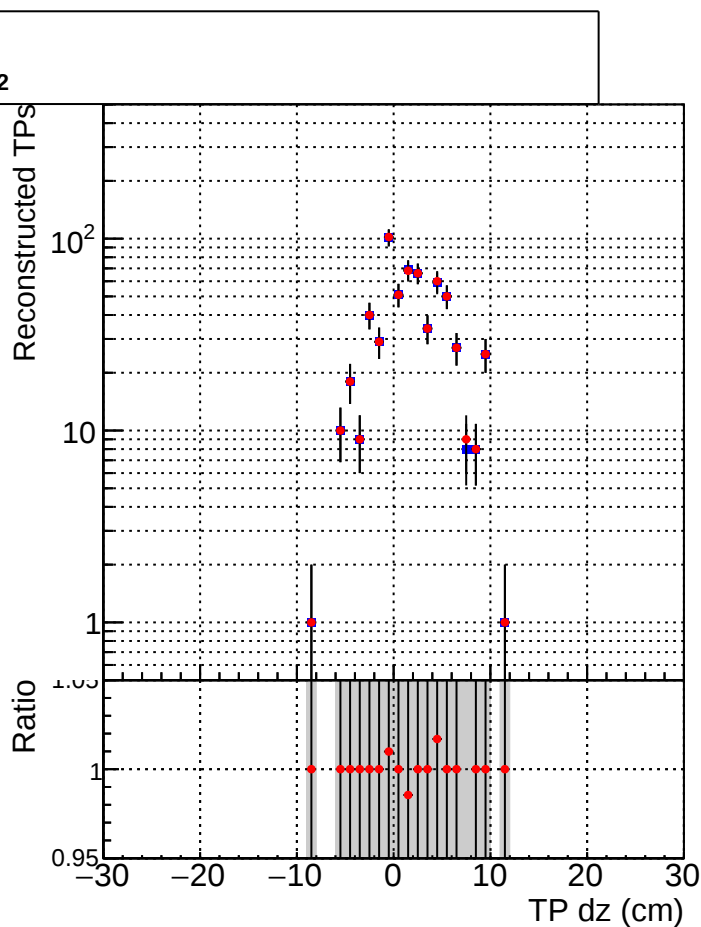
■ DQM_TT_mkFit-DQM_time_old132 ■ DQM_TT_mkFit-DQM_time_new132
