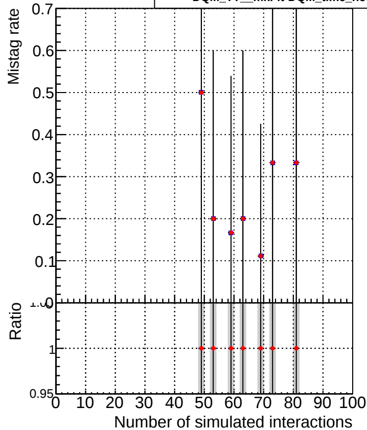
■ DQM_TT_mkFit-DQM_time_old132 ● DQM_TT_mkFit-DQM_time_new132
