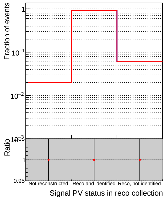
■ DQM_TT_mkFit-DQM_time_old132 ● DQM_TT_mkFit-DQM_time_new132
