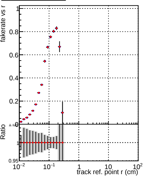
—●— DQM_TT_mkFit-DQM_time_old132 —●— DQM_TT_mkFit-DQM_time_new132
