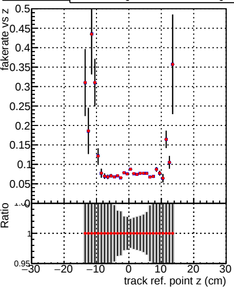
—●— DQM_TT_mkFit-DQM_time_old132 —●— DQM_TT_mkFit-DQM_time_new132
