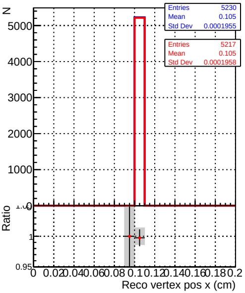
ReconstructedAllAssoc2Gen_time_old132
