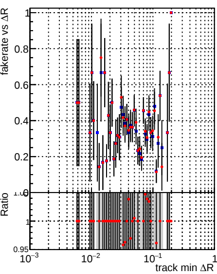
Fake rate vs \Delta R(\text{track, jet}) Legend: DQM_TT_mkFit-DQM_time_old132 (blue), DQM_TT_mkFit-DQM_time_new132 (red)
