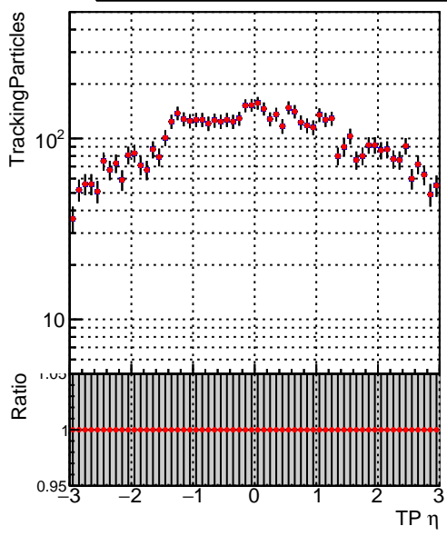
N of simulated tracks vs TP \eta Legend: - \square DQM_TT_mkFit-DQM_time_old132 - \bullet DQM_TT_mkFit-DQM_time_new132
