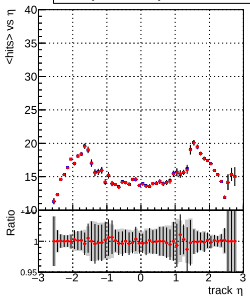
mean hits — DQM_TT_mkFit-DQM_time_old132 — DQM_TT_mkFit-DQM_time_new132
