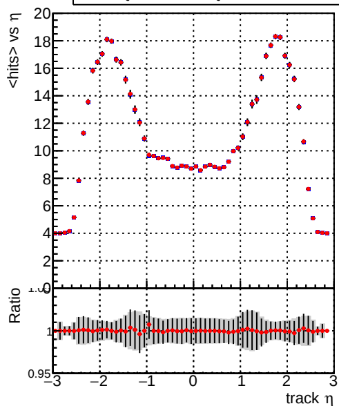
mean hits — DQM_TT_mkFit-DQM_time_old132 — DQM_TT_mkFit-DQM_time_new132
