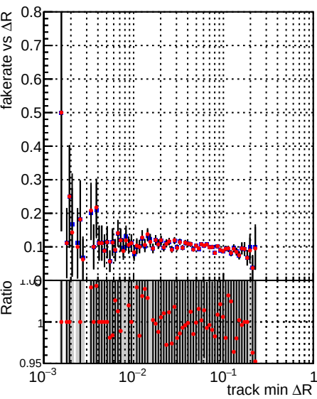
Fake rate vs \Delta R(\text{track, jet}) Legend: \blacksquare DQM_TT_mkFit-DQM_time_old132 \bullet DQM_TT_mkFit-DQM_time_new132
