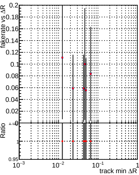
Fake rate vs \Delta R(\text{track, jet}) DQM_TT_mkFit-DQM_time_old132 DQM_TT_mkFit-DQM_time_new132
