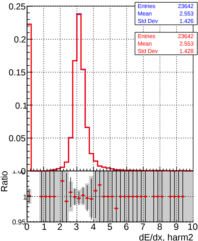
■ DQM_TT_mkFit-DQM_time_old132 ● DQM_TT_mkFit-DQM_time_new132
