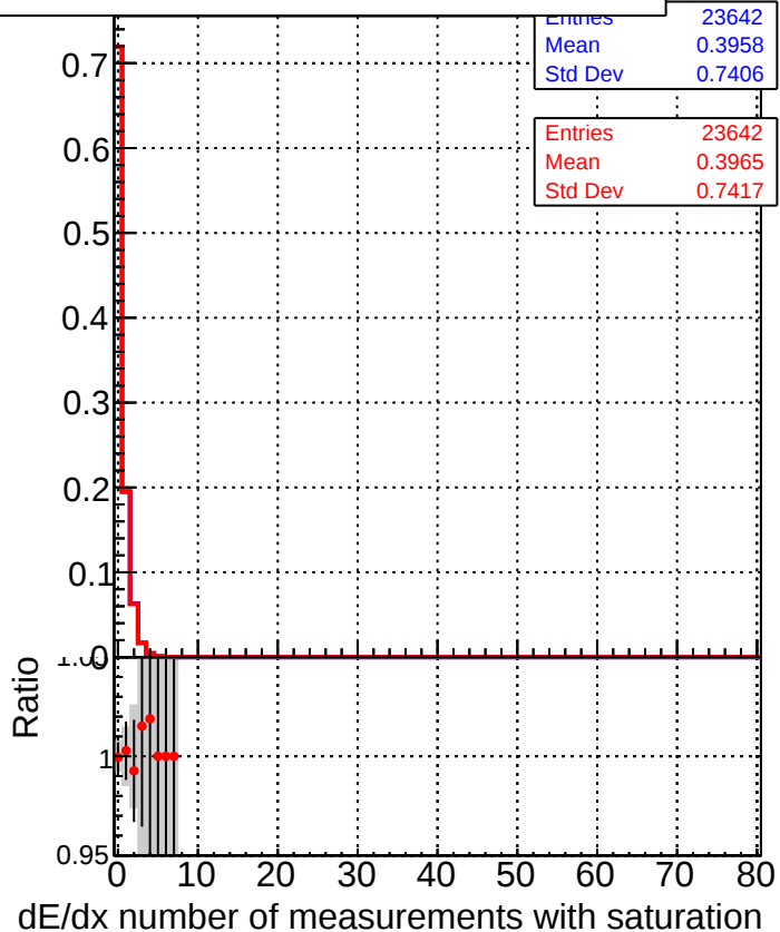
■ DQM_TT_mkFit-DQM_time_old132 ● DQM_TT_mkFit-DQM_time_new132
