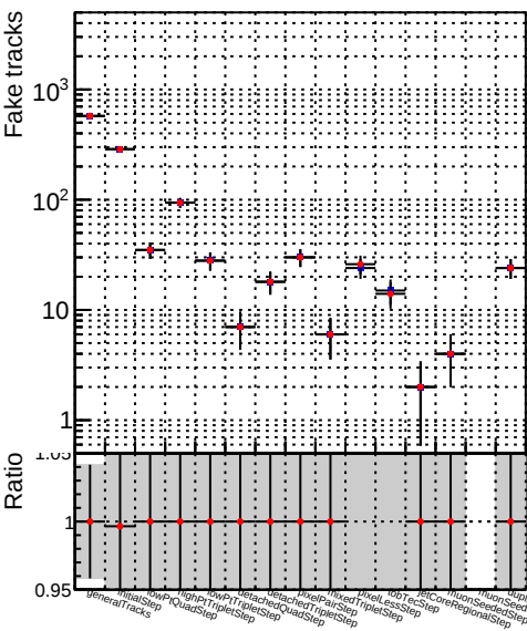
Number —●— DQM_TT_mkFit-DQM_time_new132
