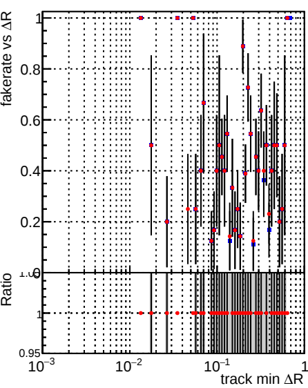
Fake rate vs \Delta R(\text{track, jet}) Legend: DQM_TT_mkFit-DQM_time_old132 (blue squares) DQM_TT_mkFit-DQM_time_new132 (red circles)
