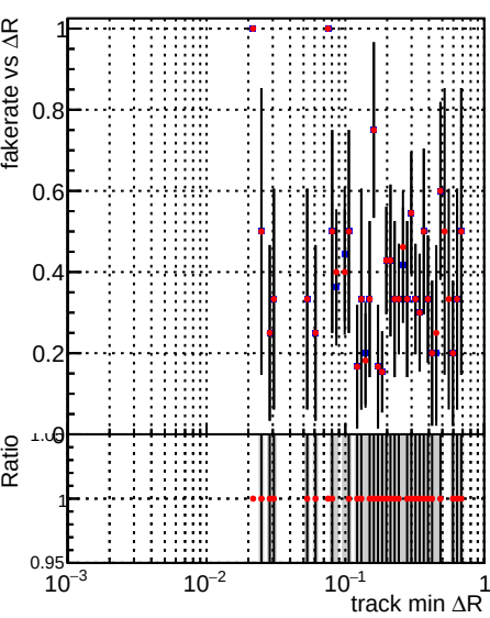
Fake rate vs \Delta R (track, jet) Legend: DQM_TT_mkFit-DQM_time_old132 (blue squares), DQM_TT_mkFit-DQM_time_new132 (red circles)
