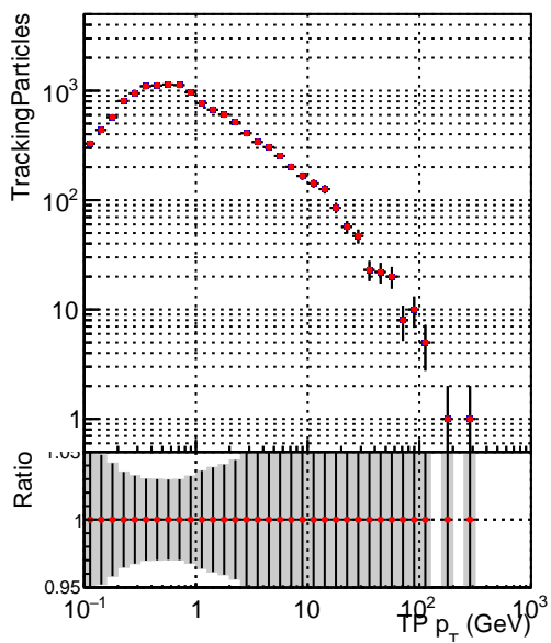
—•— DQM_TT_mkFit-DQM_time_old132 —•— DQM_TT_mkFit-DQM_time_new132
