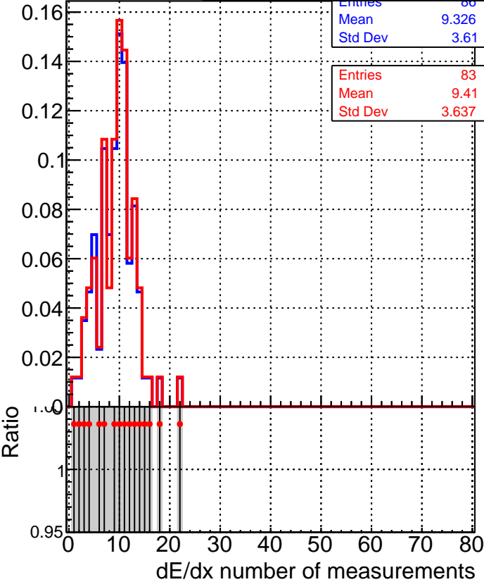
■ DQM_TT_mkFit-DQM_time_old132 ● DQM_TT_mkFit-DQM_time_new132
