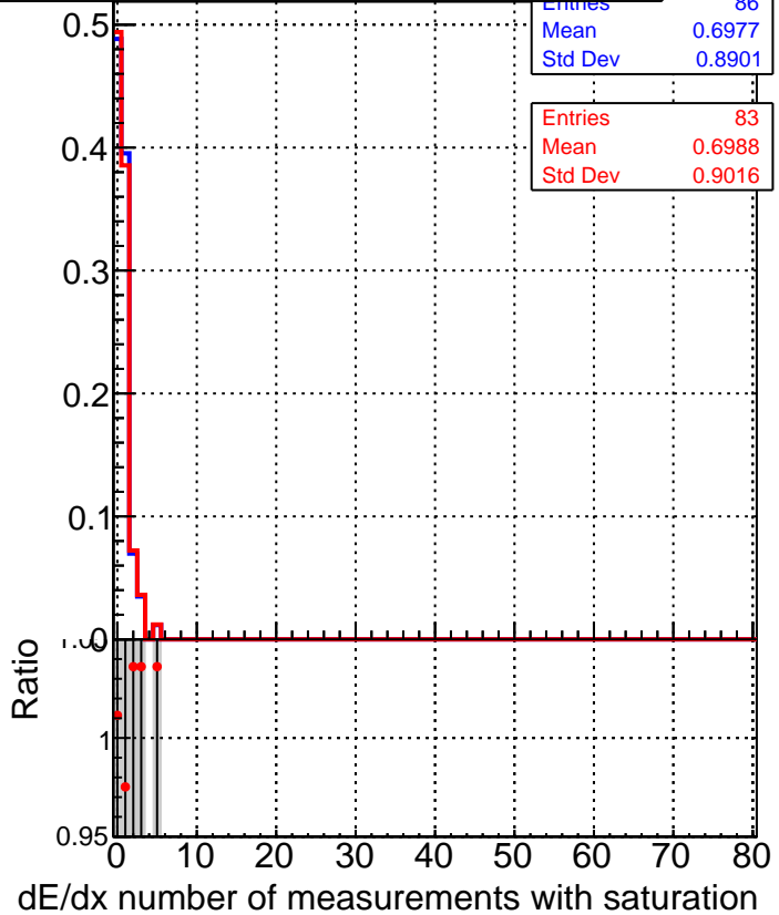
■ DQM_TT_mkFit-DQM_time_old132 ● DQM_TT_mkFit-DQM_time_new132
