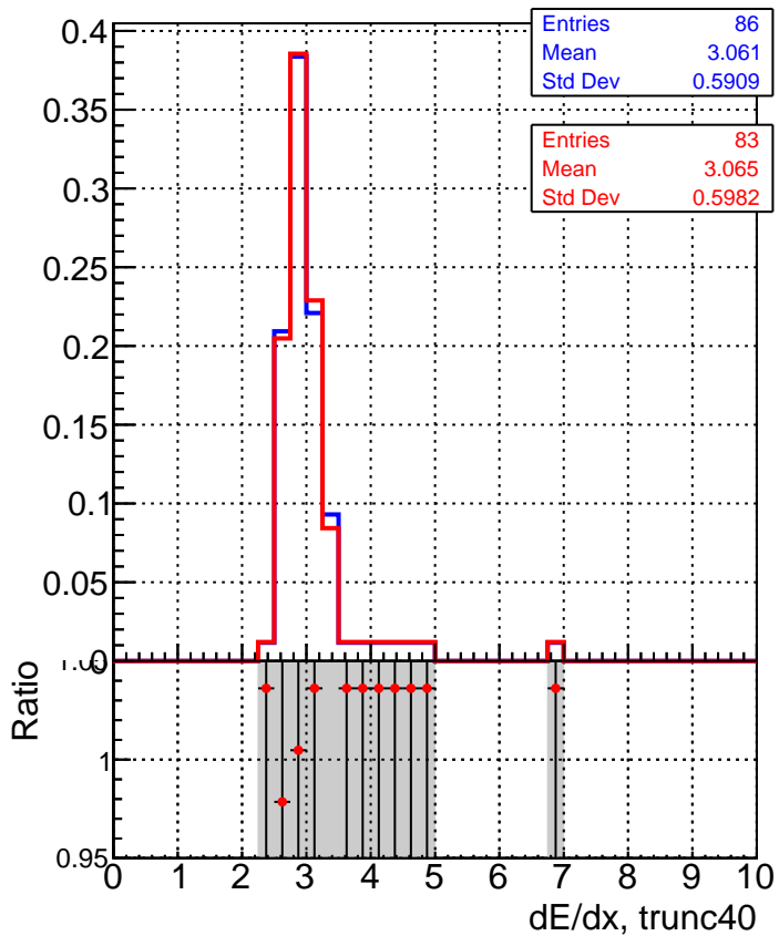
■ DQM_TT_mkFit-DQM_time_old132 ● DQM_TT_mkFit-DQM_time_new132
