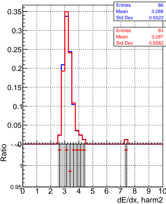
■ DQM_TT_mkFit-DQM_time_old132 ● DQM_TT_mkFit-DQM_time_new132
