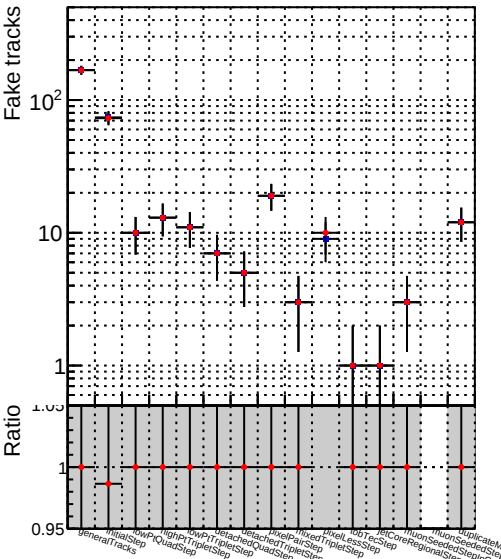
Number —●— DQM_TT_mkFit-DQM_time_new132
