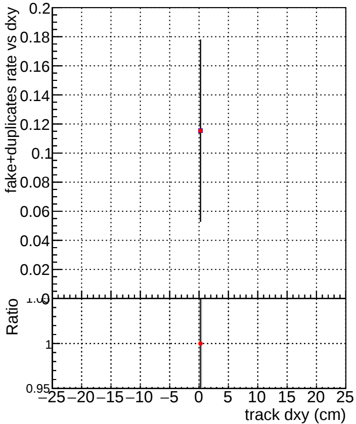
DQM_TT_mkFit-DQM_time_old132 DQM_TT_mkFit-DQM_time_new132
