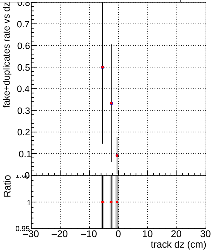
DQM_TT_mkFit-DQM_time_old132 DQM_TT_mkFit-DQM_time_new132
