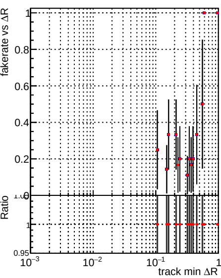
Fake rate vs \Delta R(\text{track, jet}) Legend: DQM_TT_mkFit-DQM_time_old132 (blue dots) DQM_TT_mkFit-DQM_time_new132 (red dots)
