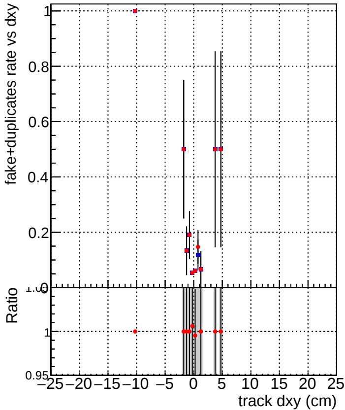
DQM_TT_mkFit-DQM_time_old132 DQM_TT_mkFit-DQM_time_new132
