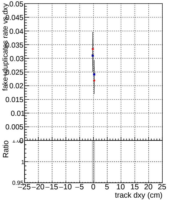
DQM_TT_mkFit-DQM_time_old132 DQM_TT_mkFit-DQM_time_new132
