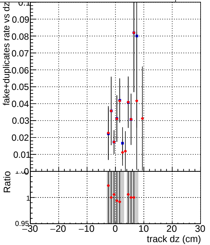
DQM_TT_mkFit-DQM_time_old132 DQM_TT_mkFit-DQM_time_new132
