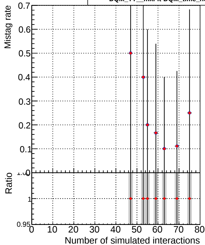
■ DQM_TT_mkFit-DQM_time_old132 ● DQM_TT_mkFit-DQM_time_new132
