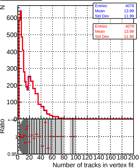
ReconstructedAllAssoc2Gen_NumTracks
