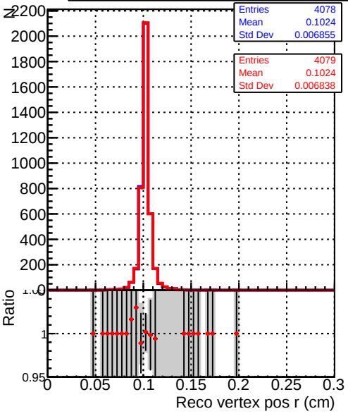
Recons DQM_TT_mkFit-DQM_time_old132 DQM_TT_mkFit-DQM_time_new132
