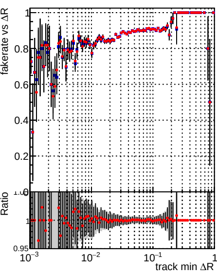
Legend: DQM_TT_mkFit-QM_time_old132 (blue), DQM_TT_mkFit-QM_time_new132 (red)
