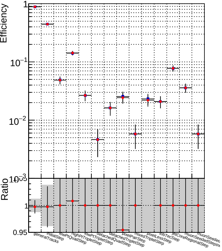
DQM_TT_mkFit-DQM_time_old132 DQM_TT_mkFit-DQM_time_new132
