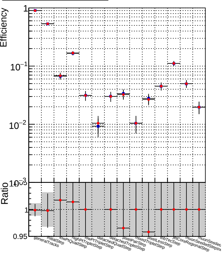
DQM_TT_mkFit-DQM_time_old132 DQM_TT_mkFit-DQM_time_new132
