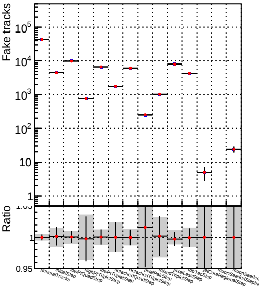
Number —●— DQM_TT_mkFit-DQM_time_new132
