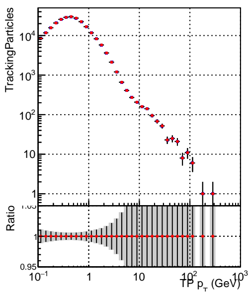
— DQM_TT_mkFit-DQM_time_old132 — DQM_TT_mkFit-DQM_time_new132
