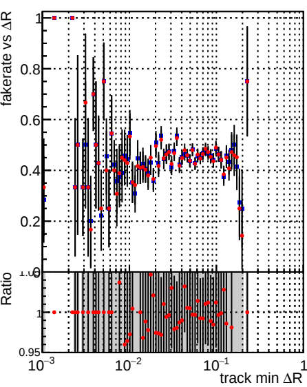
Legend: DQM_TT_mkFit-DQM_time_old132 (blue), DQM_TT_mkFit-DQM_time_new132 (red)
