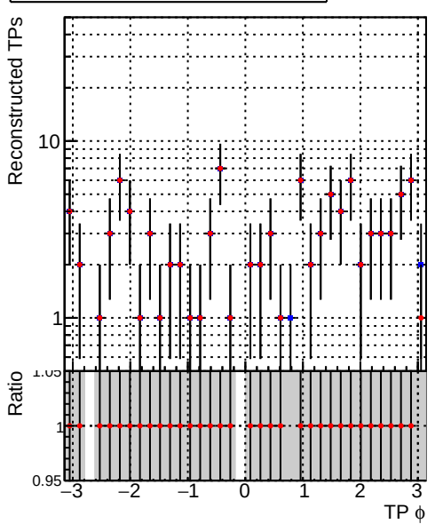
N of associated tracks (simToReco) vs TP \phi
