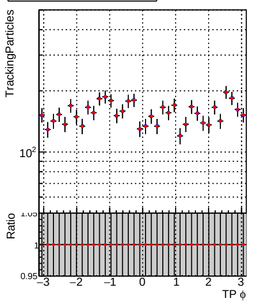
N of simulated tracks vs TP \phi
