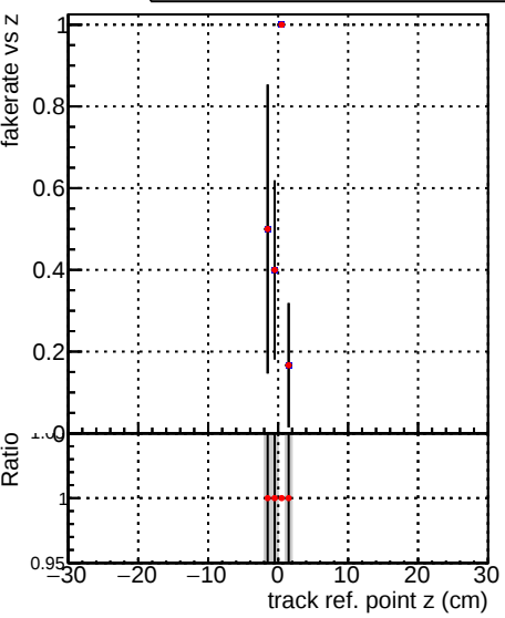
Fake rate vs verpos DQM_TT_mkFit-DQM_time_old132 DQM_TT_mkFit-DQM_time_new132
