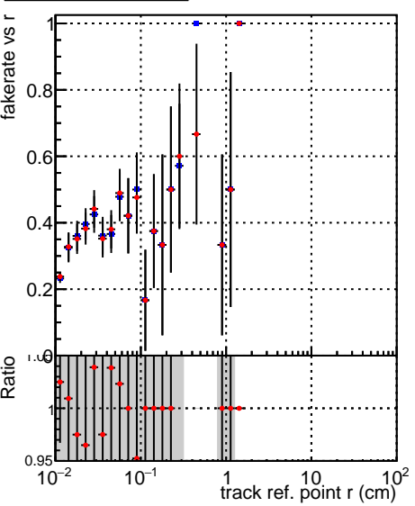
◆ DQM_TT_mkFit-DQM_time_old132 ● DQM_TT_mkFit-DQM_time_new132
