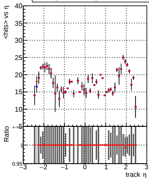
mean hits vs \eta DQM_TT_mkFit-DQM_time_old132 DQM_TT_mkFit-DQM_time_new132
