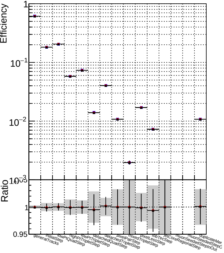
DQM_TT_mkFit-DQM_old132 DQM_TT_mkFit-DQM_new132 DQM_TT_mkFit-DQM_newfast132
