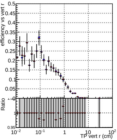
Efficiency vs vertpos DQM_TT_mkFit-DQM_old132 DQM_TT_mkFit-DQM_new132 DQM_TT_mkFit-DQM_newfast132
