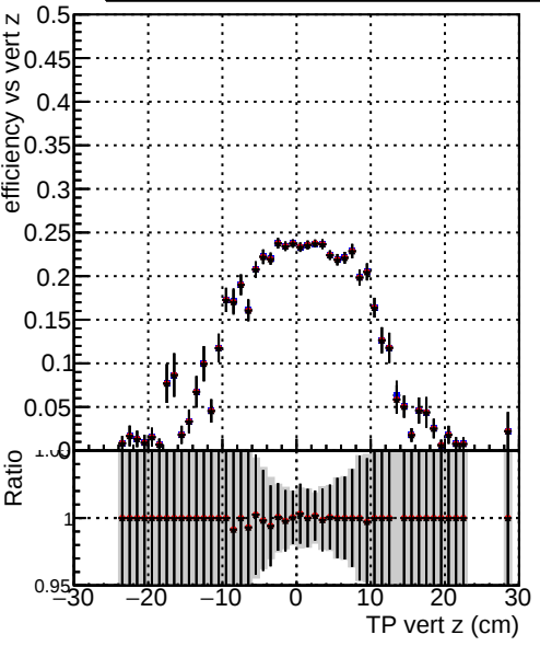
Efficiency vs TP vert z (cm) Legend: DQM_TT_mkFit-DQM_old132 DQM_TT_mkFit-DQM_new132 DQM_TT_mkFit-DQM_newfast132
