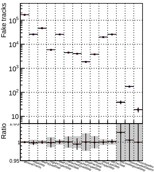
Number DQM_TT_mkFit-DQM_new132 DQM_TT_mkFit-DQM_newfast132
