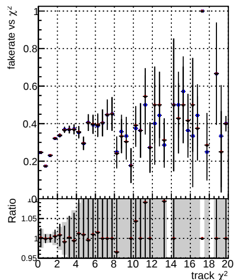
Fake rate vs. Model Color Shape DOM TT mkFit-DOM-old132 Blue Circle DOM TT mkFit-DOM-new132 Red Circle DOM TT mkFit-DOM-newrast132 Black Circle
