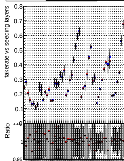
Fake rate vs. Model Color Shape DOM TT mkFit-DOM-old132 Blue Circle DOM TT mkFit-DOM-new132 Red Circle DOM TT mkFit-DOM-newrast132 Black Circle
