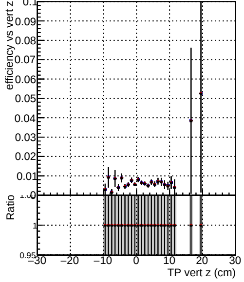
Efficiency vs. TP vert z (cm) Legend: - DQM_TT_mkFit-DQM_old132 (blue line with circles) - DQM_TT_mkFit-DQM_new132 (red line with circles) - DQM_TT_mkFit-DQM_newfast132 (black line with circles)
