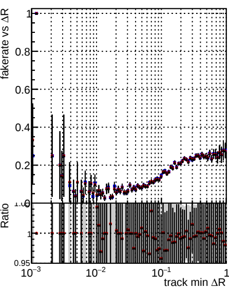
Fake rate vs \Delta R(\text{track, jet}) Legend: DQM TT mkFit-DQM old132 (black dots) DQM TT mkFit-DQM new132 (blue dots) DQM TT mkFit-DQM newfast132 (red dots)
