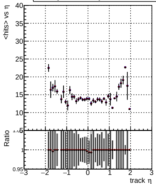
mean hit DQM_TT_mkFit-DQM_old132 DQM_TT_mkFit-DQM_new132 DQM_TT_mkFit-DQM_newfast132
