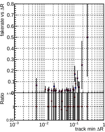
Fake rate vs ΔR(track, jet) Legend: DQM TT mkFit-DQM old132 (blue dots) DQM TT mkFit-DQM new132 (red dots) DQM TT mkFit-DQM newfast132 (black dots)
