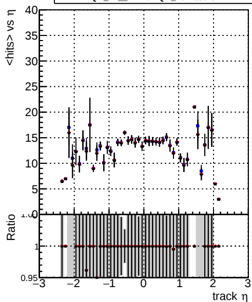
mean hit — DQM_TT_mkFit-DQM_old132 — DQM_TT_mkFit-DQM_new132 — DQM_TT_mkFit-DQM_newfast132
