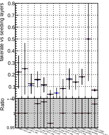
Fake rate vs. Legend: DOM TT mkFit-DOM-old132, DOM TT mkFit-DOM-new132, DOM TT mkFit-DOM-newrast132
