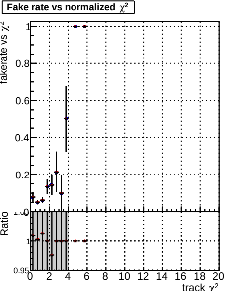
Fake rate vs. Legend: DOM TT mkFit-DOM-old132, DOM TT mkFit-DOM-new132, DOM TT mkFit-DOM-newrast132
