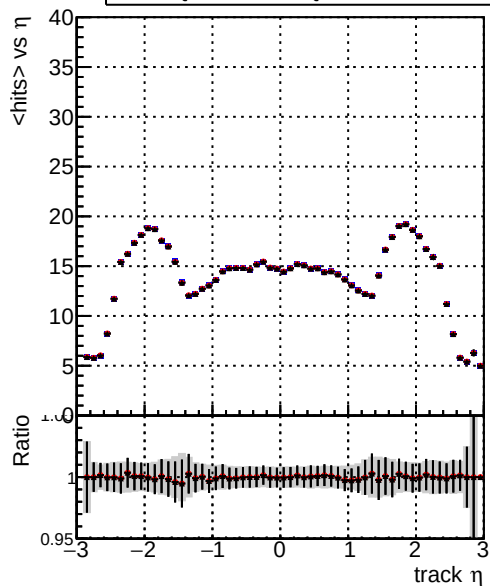
mean hits vs \eta — DQM_TT_mkFit-DQM_old132 — DQM_TT_mkFit-DQM_new132 — DQM_TT_mkFit-DQM_newfast132
