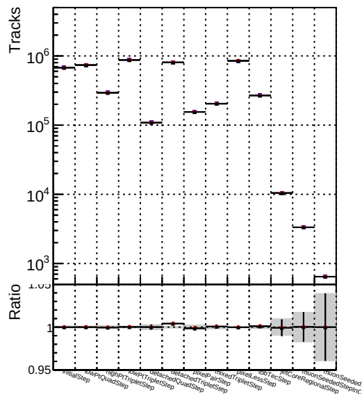
—●— DQM_TT_mkFit-DQM_old132 —●— DQM_TT_mkFit-DQM_new132 —●— DQM_TT_mkFit-DQM_newfast132
