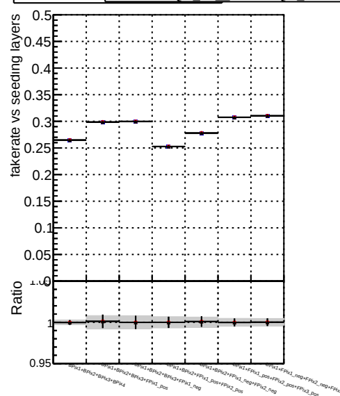
Fake rate vs. DOM TT mkFit-DOM-old132 DOM TT mkFit-DOM-new132 DOM TT mkFit-DOM-newfast132
