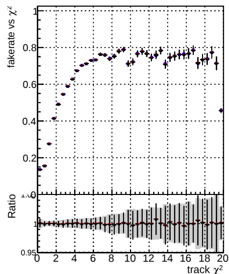
Fake rate vs. DOM TT mkFit-DOM-old132 DOM TT mkFit-DOM-new132 DOM TT mkFit-DOM-newfast132
